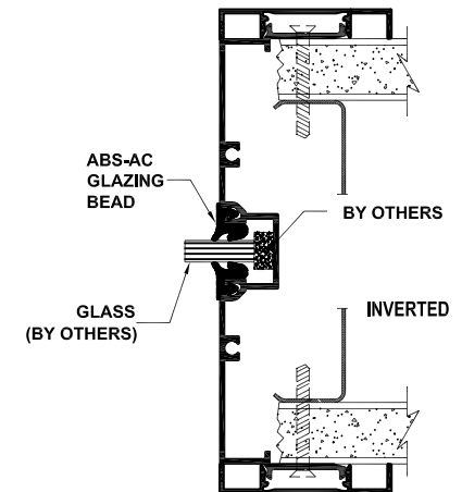
F GLAZING RAIL
