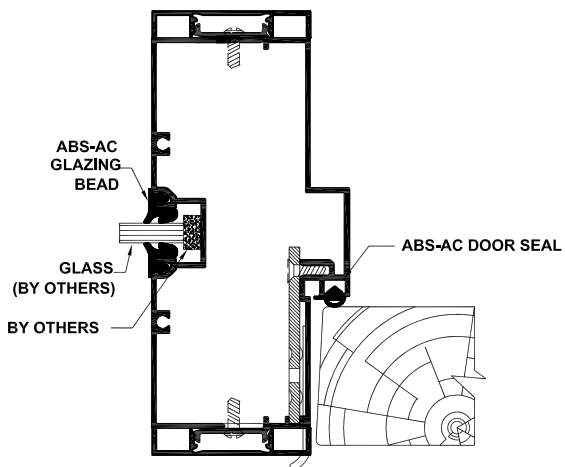
D STRIKE JAMB & S.L. MULLION W/ 2" FACE NOTE: EXTENDED LIP STRIKE NOT REQUIRED
